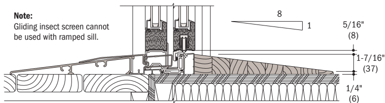
Vertical Section
